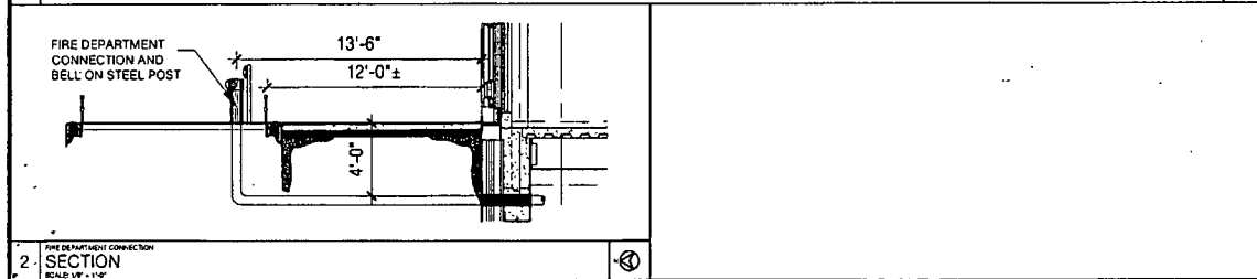
2 FIRE DEPARTMENT CONNECTION SECTION SCALE: 1/4" = 1'-0"
