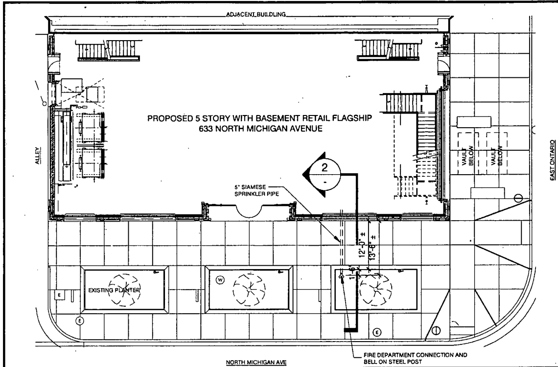
1 EXISTING PLANTERS SITE PLAN SCALE: 1/8" = 1'-0"
