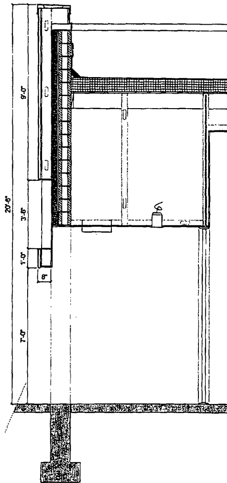
2 WALL SECTION A1.0
