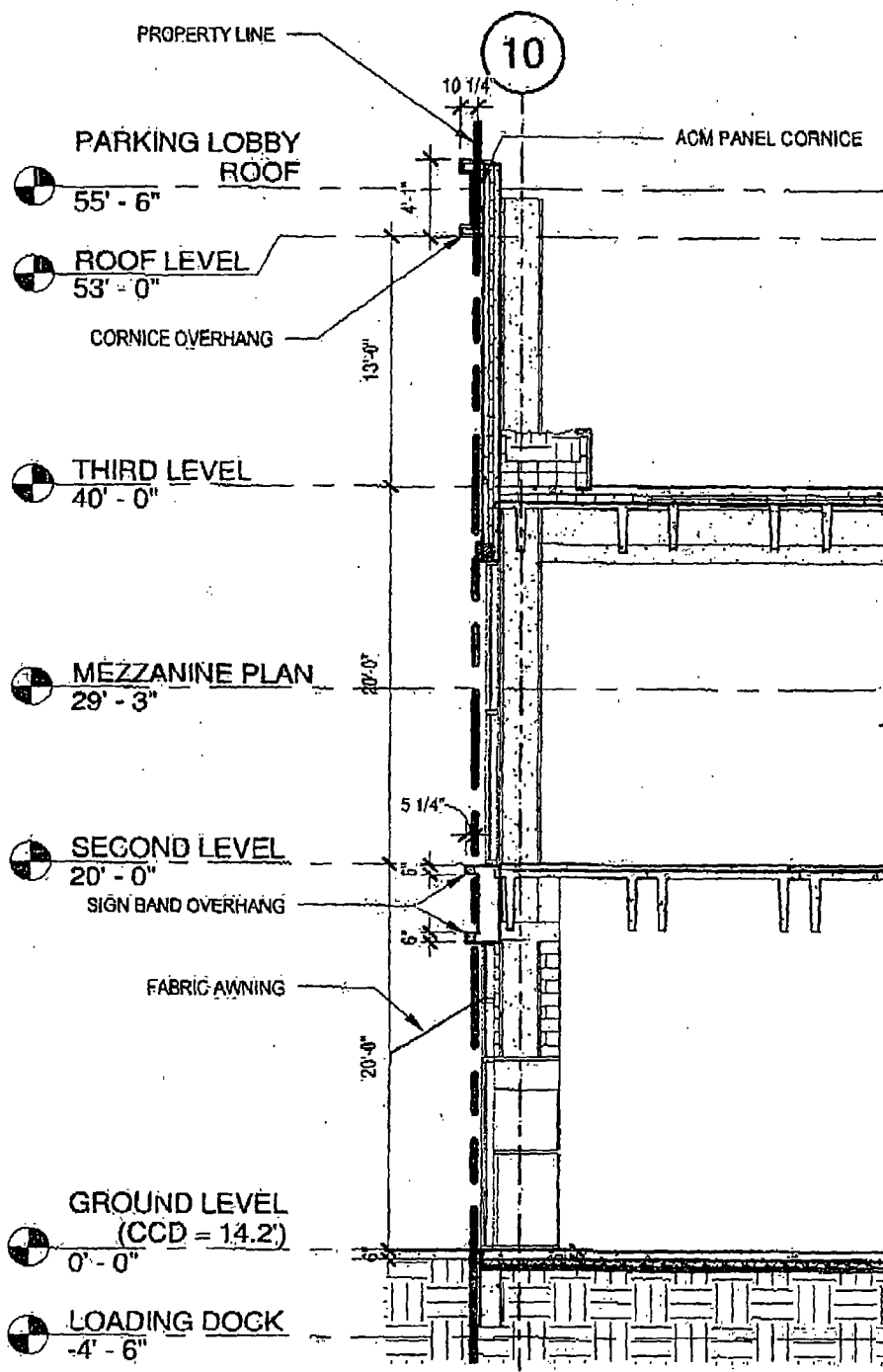
1 PUBLIC WAY USE - MONROE ST. SECTION A2-11/ASK-048 1/8" = 1'-0"
