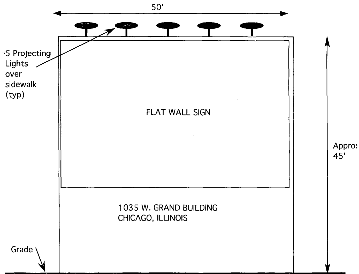
Front Elevation
