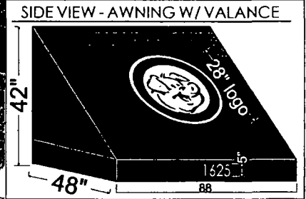
SIDE VIEW - AWNING W/ VALANCE
