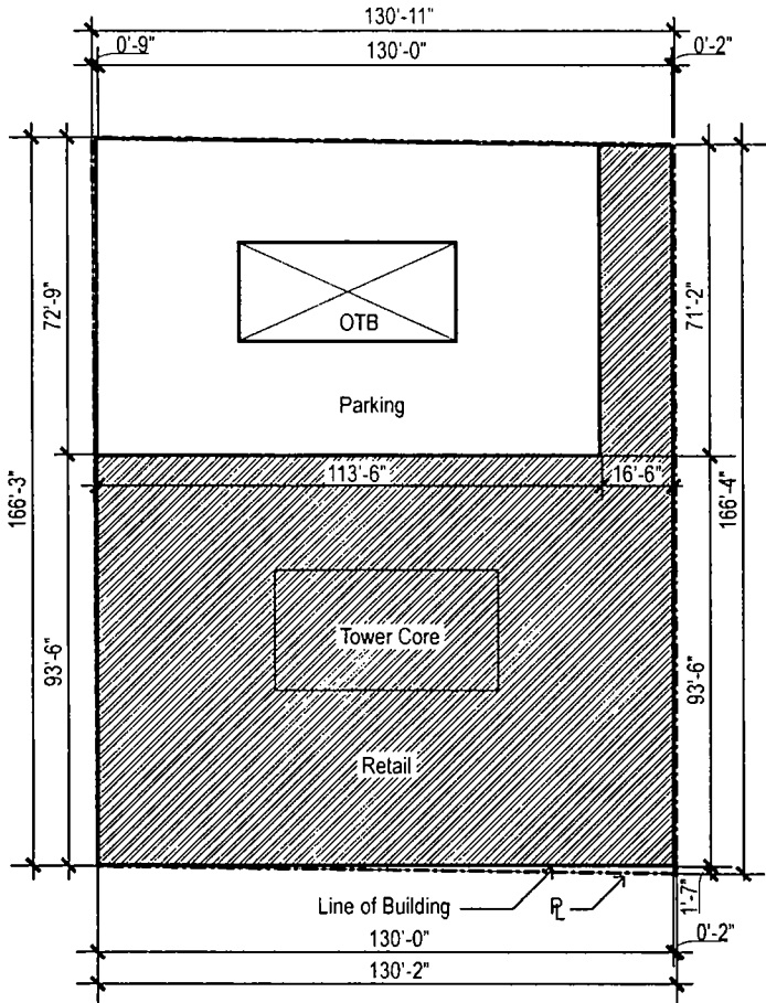
LEVEL 2 PLAN DIAGRAM
