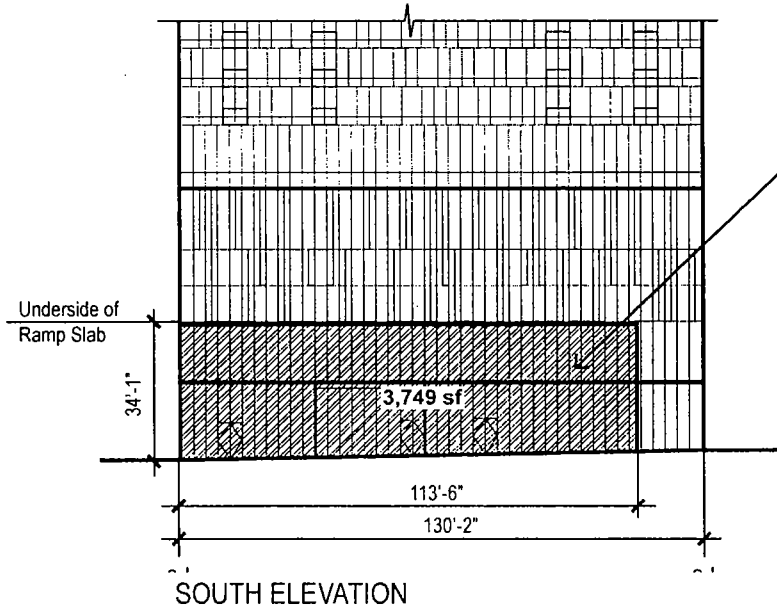
EXHIBIT 1.2 PARKING CONCEALED BY OCCUPIABLE SPACES Scale: N.T.S.
