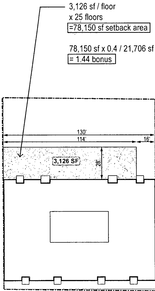
PLAN DIAGRAM
