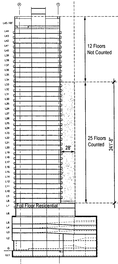
SECTION DIAGRAM
