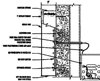
STANDARD LED ILLUMINATED CHANNEL LETTER
