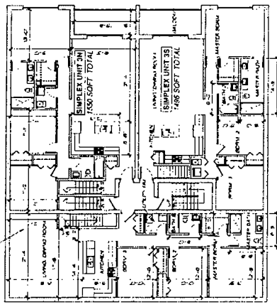
3 3RD FLOOR PLAN 3/11/12
