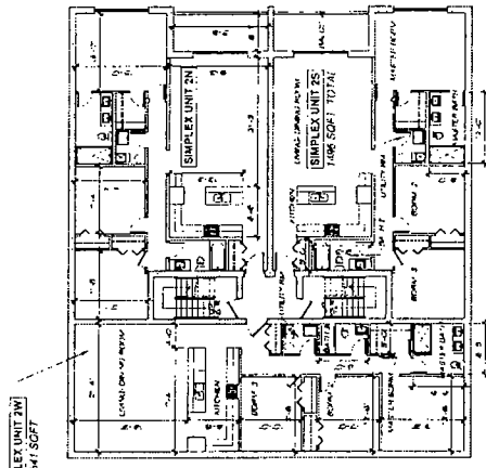
4 2ND FLOOR PLAN 3/11/12
