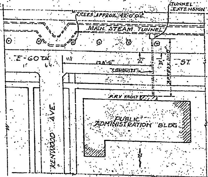
PART PLOT PLAN SCALE 1"=50'-0"
