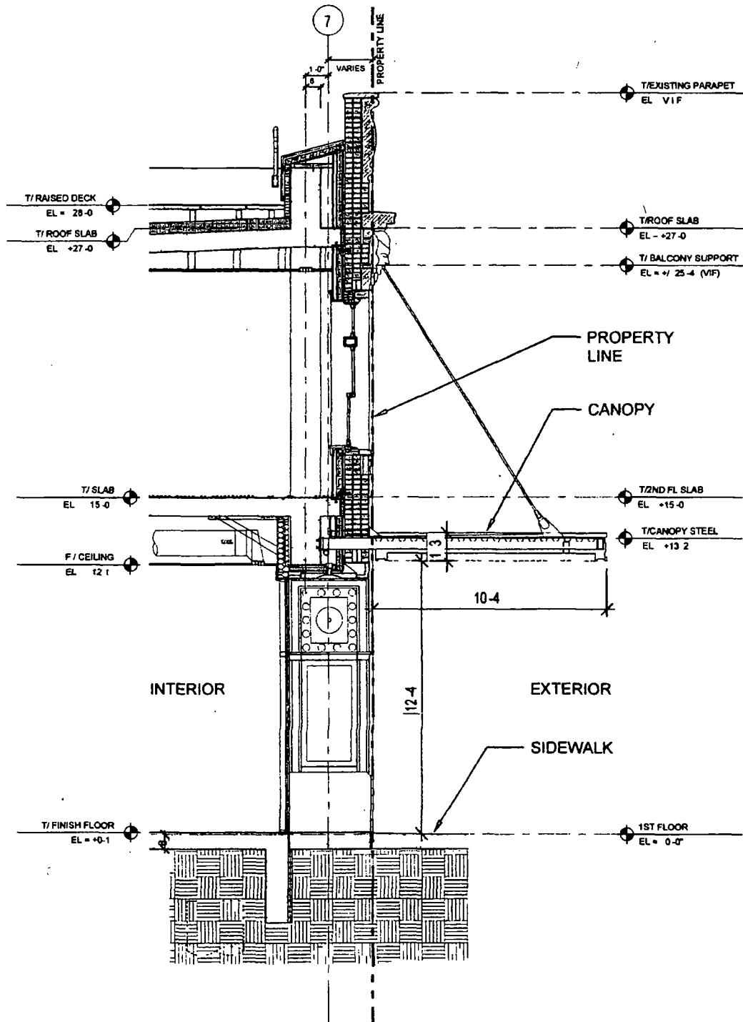
A2 SECTION CANOPY 1/4" = 1'-0"
