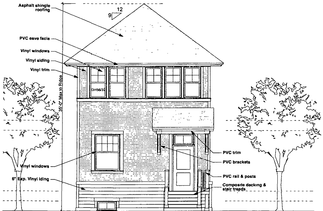
Typical Rear Elevation
