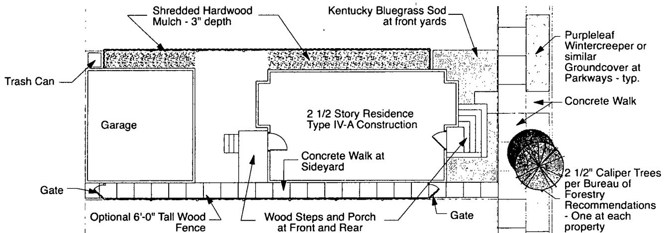
Typical 2-Car Garage Site Plan
