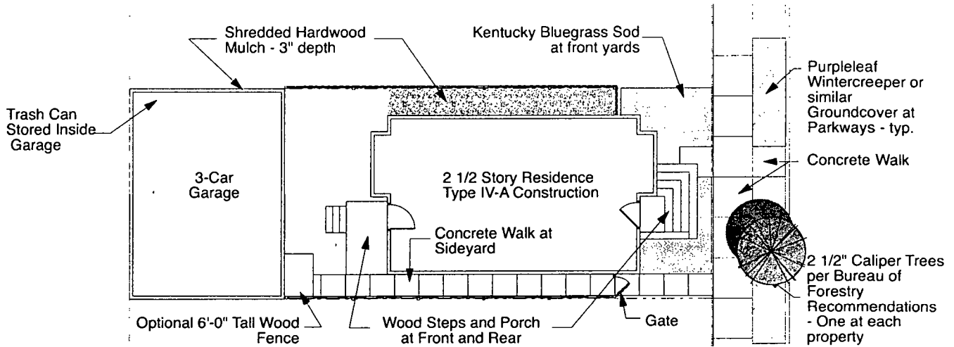
Typical 3-Car Garage Option Site Plan
