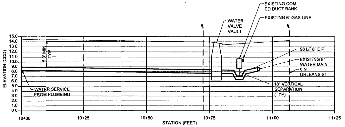
6 WATER SERVICE PROFILE SCALE V 1" = 5' H 1" = 10'
