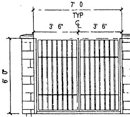
2 ASK 001A ELEVATION 1/4" = 1'-0"
