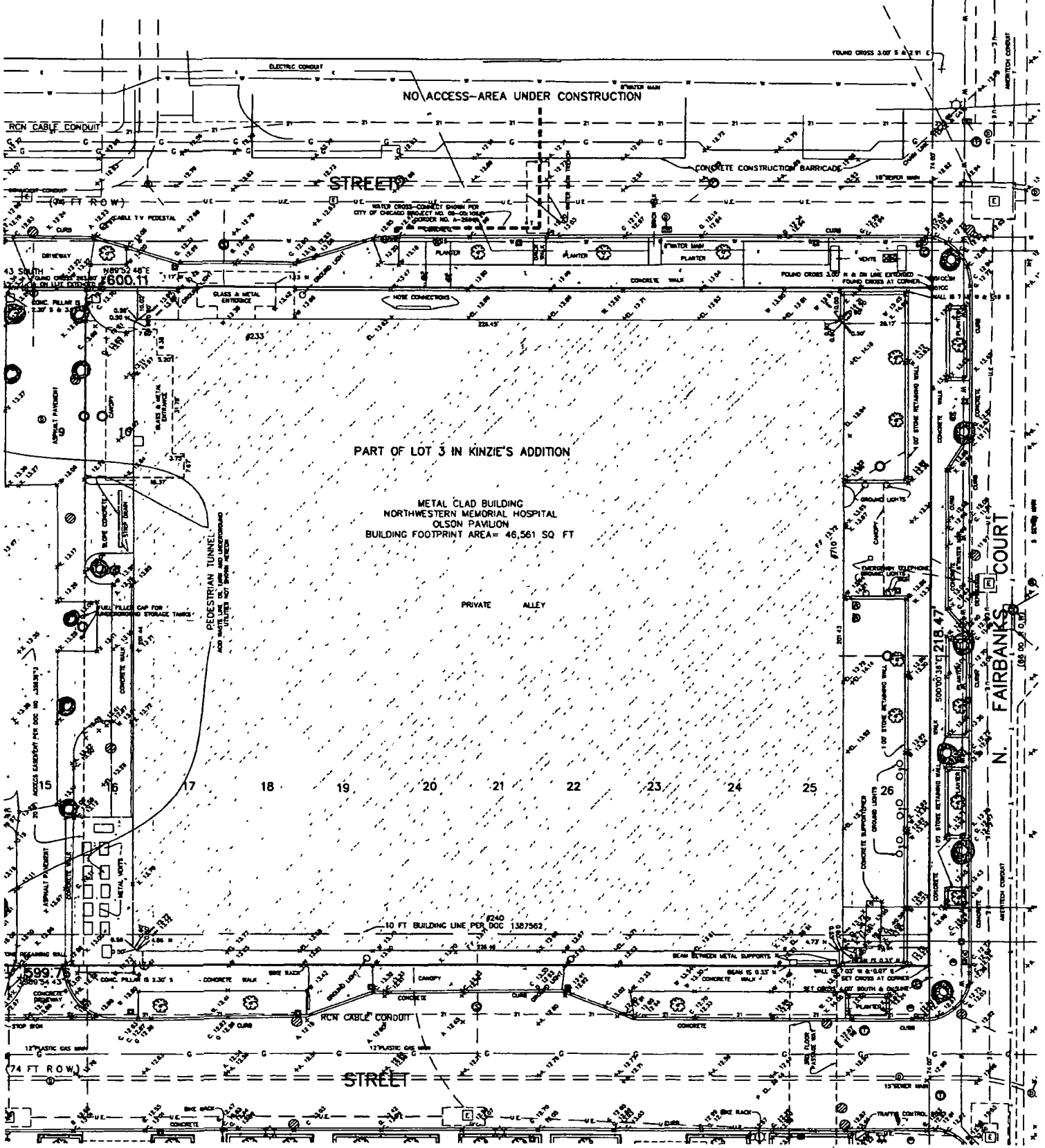
SITE PLAN LIGHT FIXTURE PWL # 109695B
