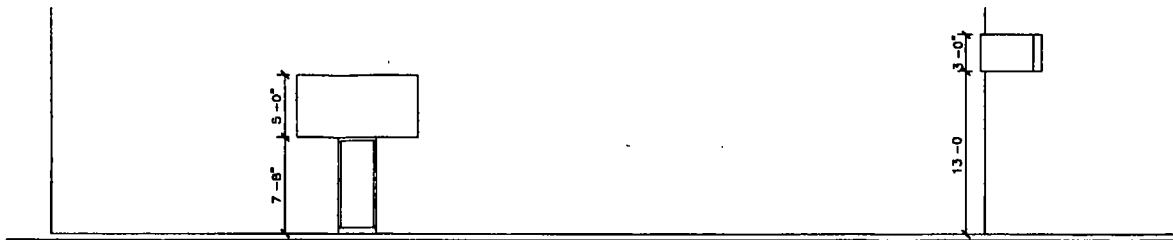
○ 200 W OHIO—OHIO STREET ELEVATION SCALE 3/32 = 1'-0"
