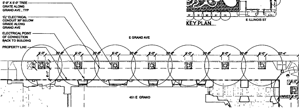
GOP-SK-001: TREE GRATES - E GRAND AVE. SCALE 1/4" = 1'-0"
