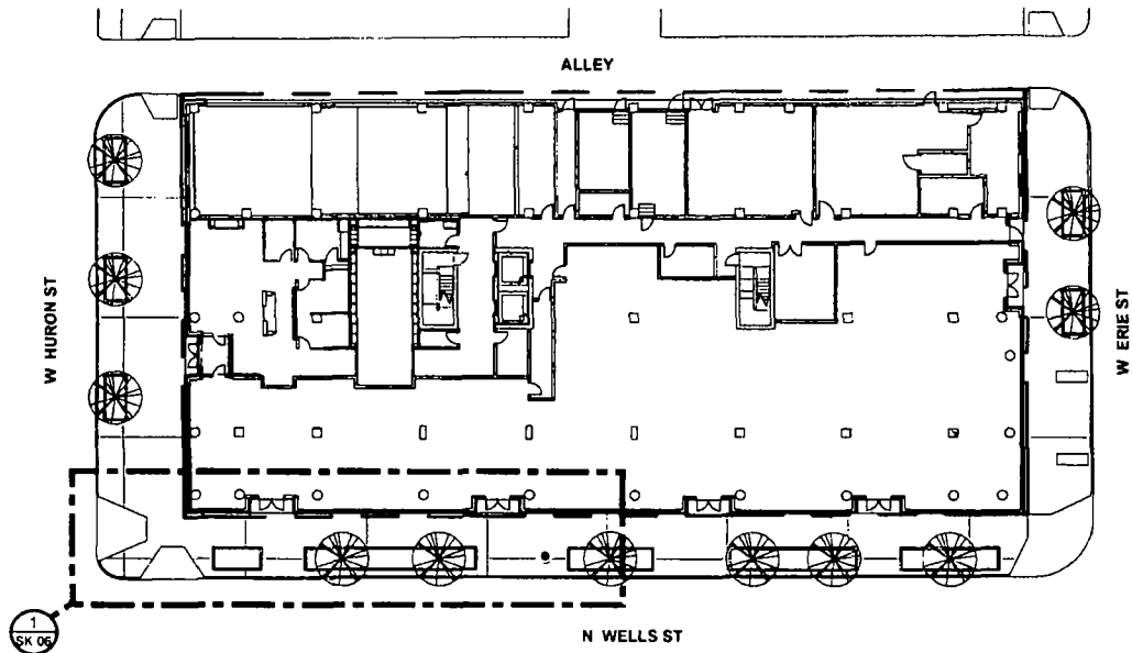
2 Site Plan PWU SK 06 1" = 50'-0"
