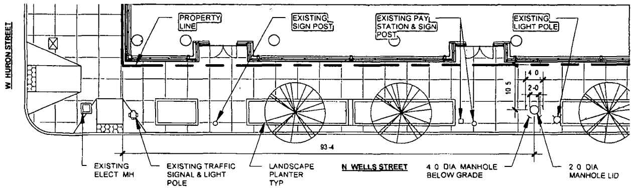
1 Enlarged Site Plan at Manhole PWU SK 06 1" = 20'-0"
