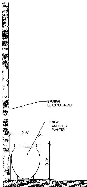
2 PLANTER ELEVATION
