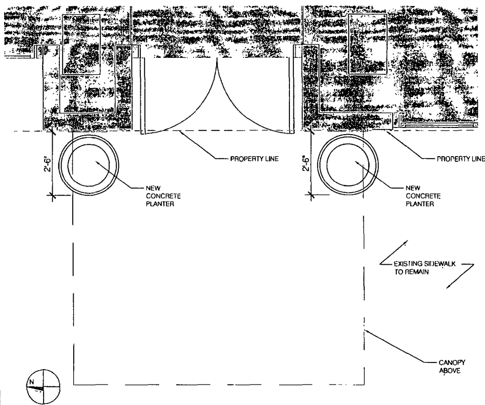
1 PLANTER PLAN
