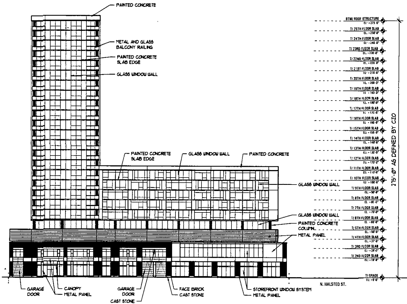
1 SOUTH ELEVATION SCALE: 1" = 50'-0"
