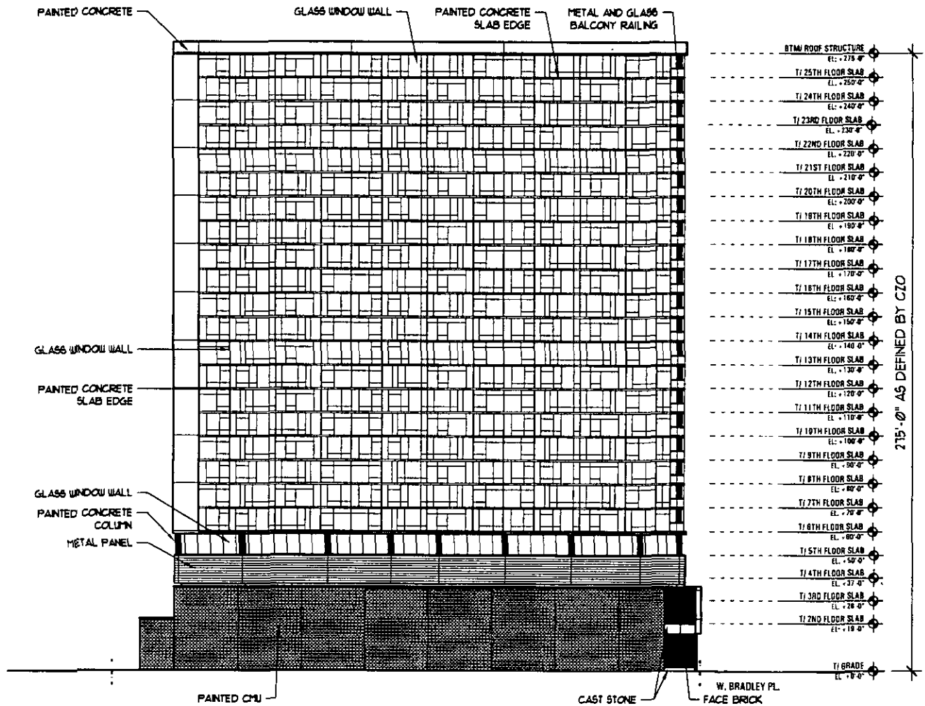
1 WEST ELEVATION SCALE: 1" = 50'-0"
