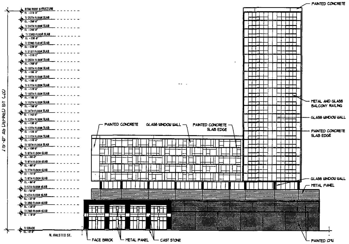
1 NORTH ELEVATION SCALE: 1" = 50'-0"
