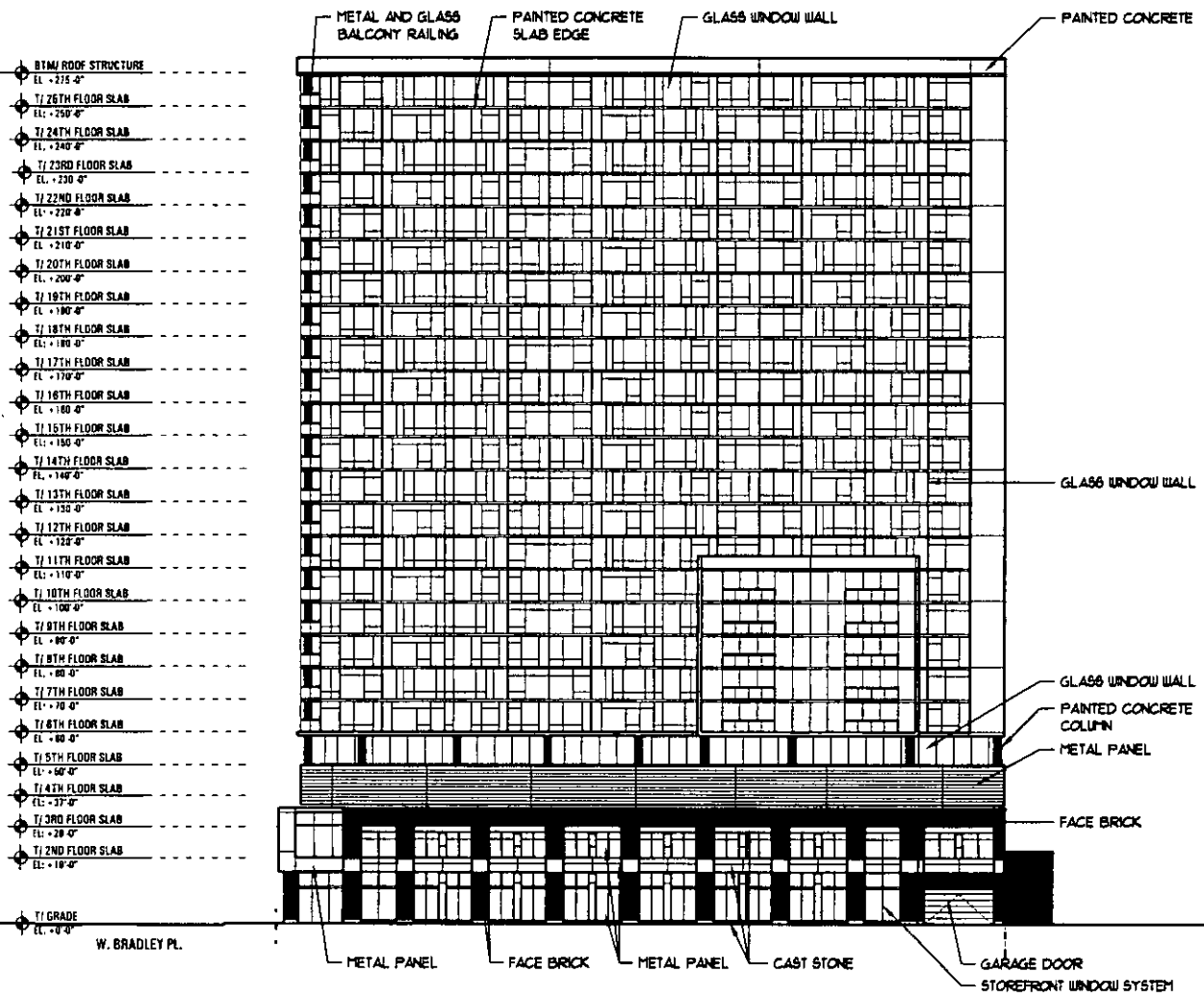
1 EAST ELEVATION SCALE: 1" = 50'-0"
