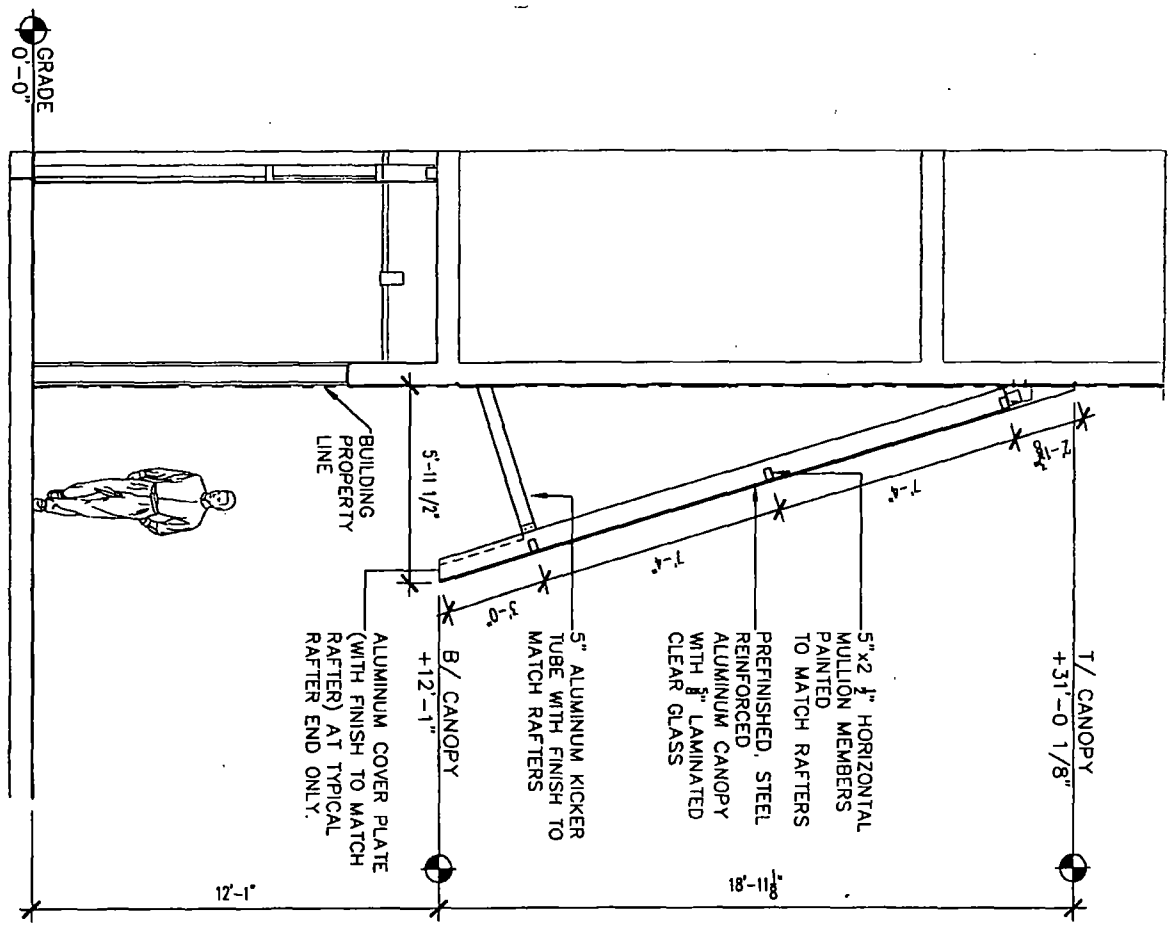
2 SECTION OF CANOPY
