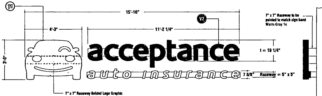
"ACCEPTANCE" LED Face Lit Letter Mounted on (Raceway)
