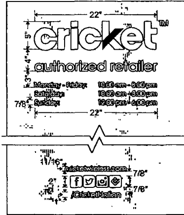
Vinyl Details 1-1/2" = 1'
