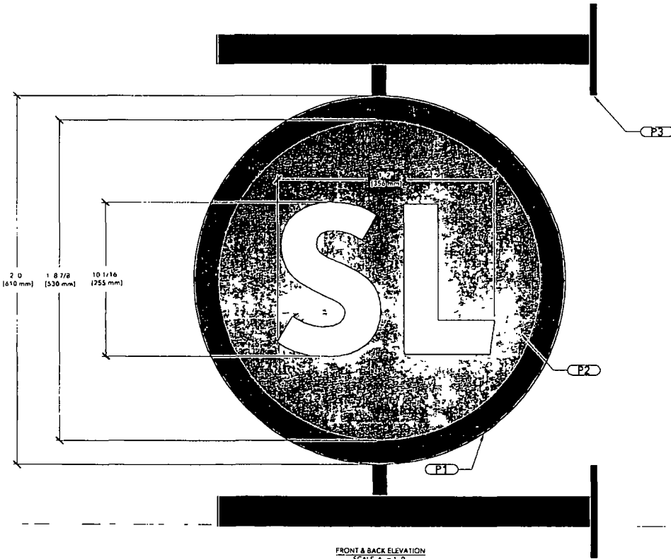
FRONT & BACK ELEVATION SCALE 6 = 1 0
