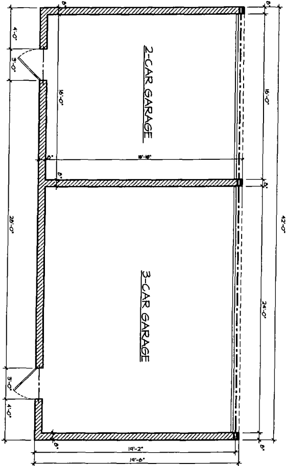
GARAGE FLOOR PLAN
