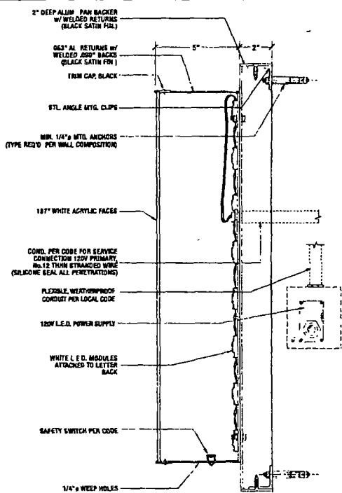
(A) TYPICAL FACE-LIT CHANNEL LETTER w/ ALUM. PAN SCALE 3/8"=1'
