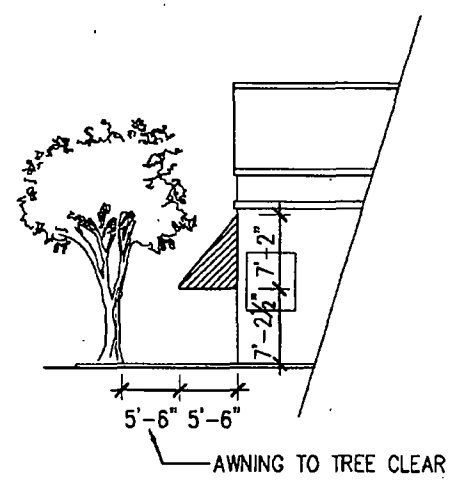
3 SIDE ELEVATION (TYP)
