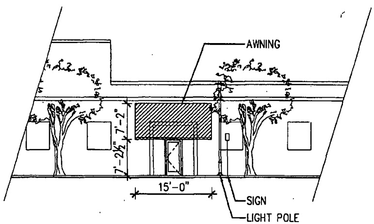
2 FRONT ELEVATION
