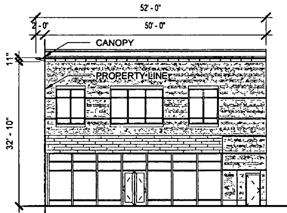
SOUTHPORT AVE ELEVATION
