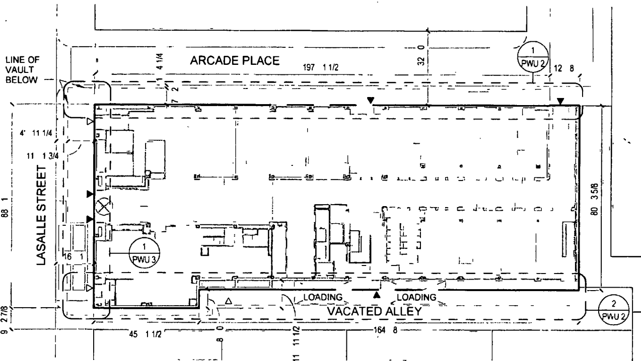
1 SITE PLAN 1" = 30' 0"
