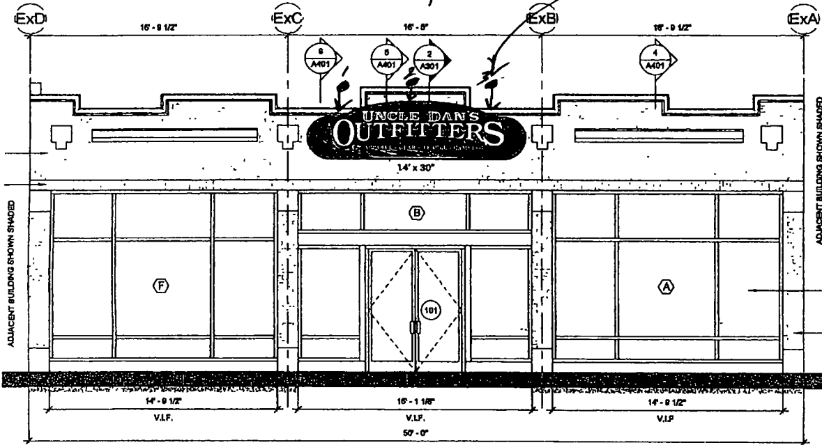
4 EAST ELEVATION 201 Scale: 1/4" = 1'-0" * Sign Panel sign panel 30" x 14'
