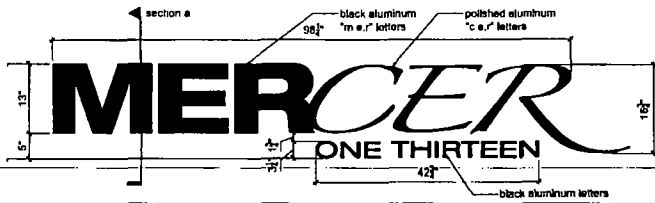
sign - front elevation
