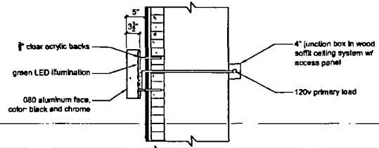
a detail sign section
