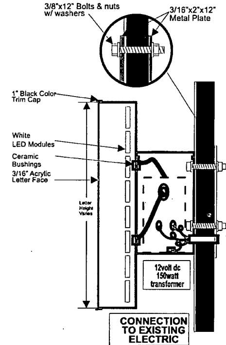
CHANNEL LETTER DETAIL NOT SCALE
