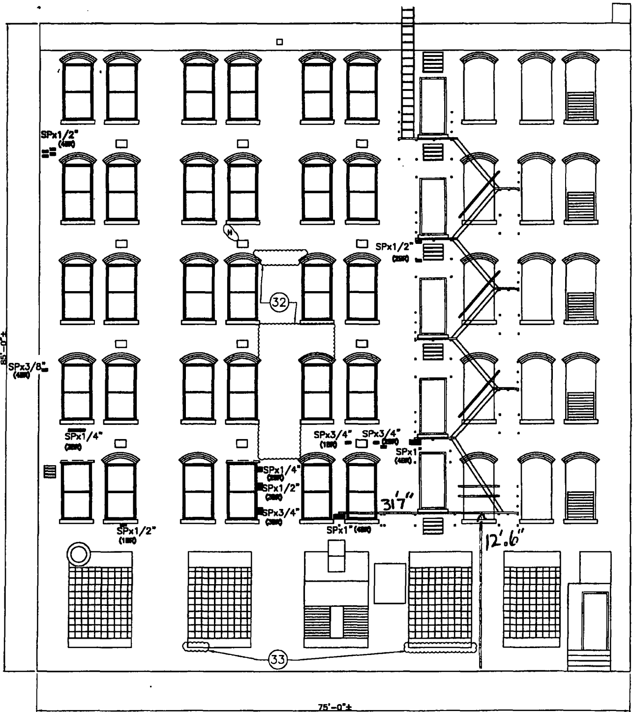
NORTH ELEVATION LOOKING SOUTH
