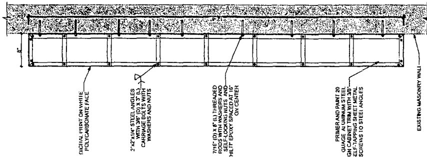
1 A-1 BOX SIGN SECTION NOT TO SCALE
