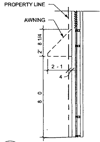
3 SIDE ELEVATION - AWNING 1 pg 03 SCALE 1/4" = 1'-0"
