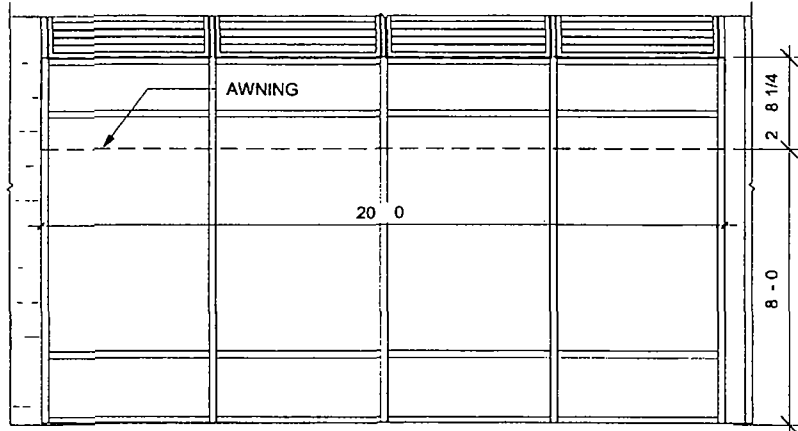
2 FRONT ELEVATION - AWNING 1 pg 03 SCALE 1/4" = 1'-0"
