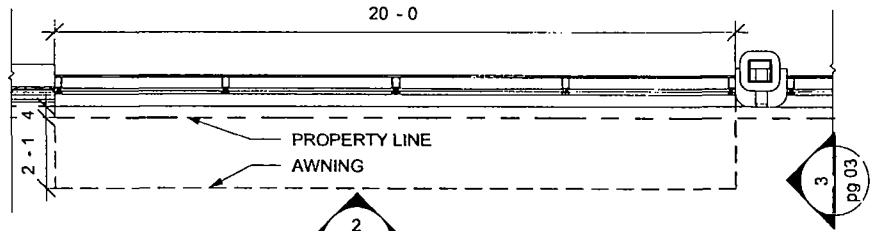
1 PLAN - AWNING 1 pg 03 SCALE 1/4" = 1'-0"
