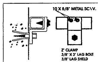
FRAME TO WALL ANCHOR DETAIL
