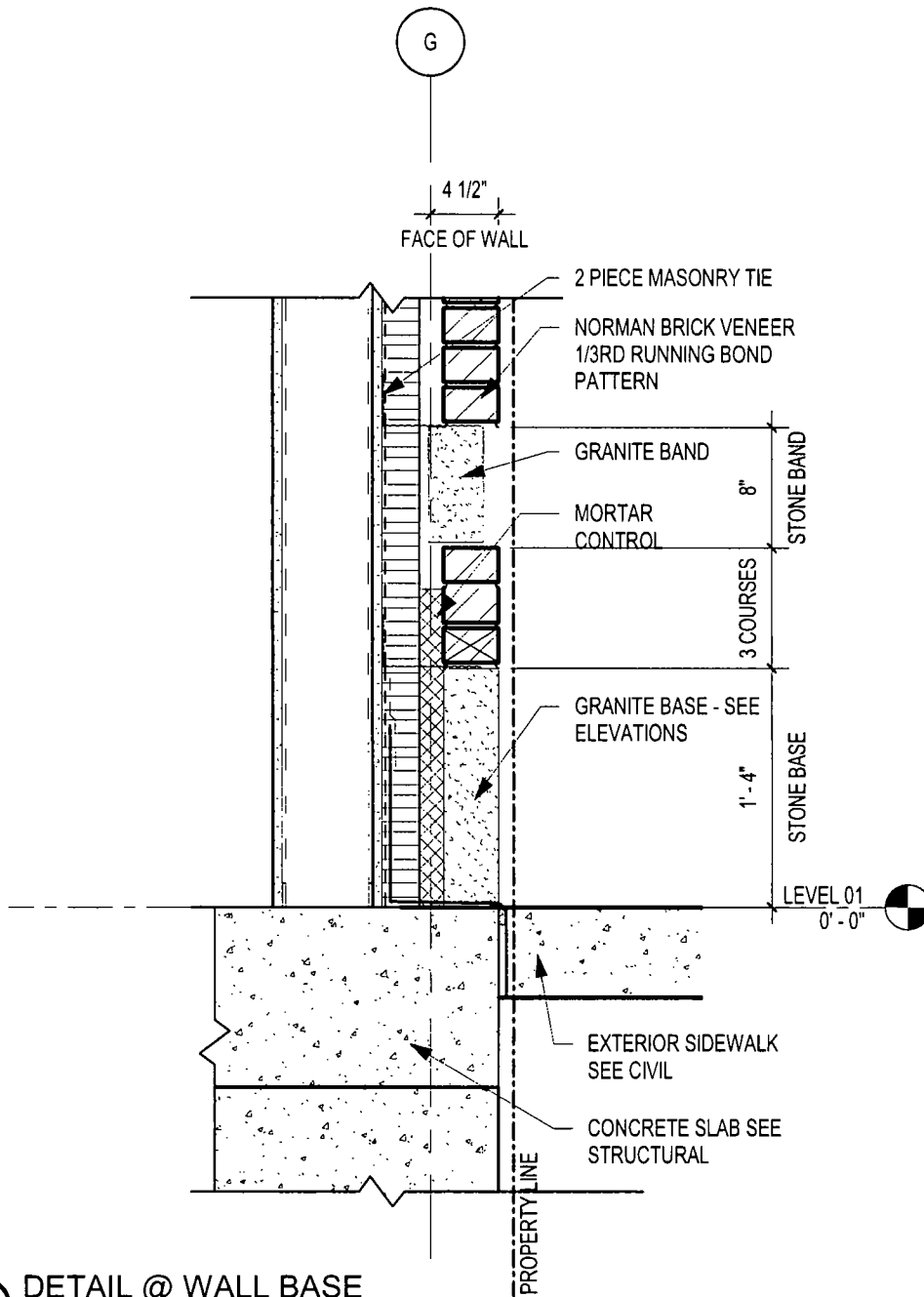
① DETAIL @ WALL BASE 1" = 1'-0"
