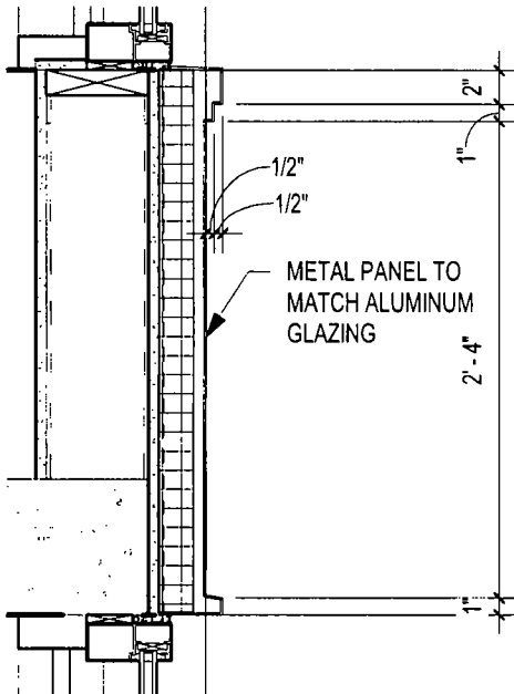
① DETAIL @ TYPICAL SPANDRAL 1" = 1'-0"
