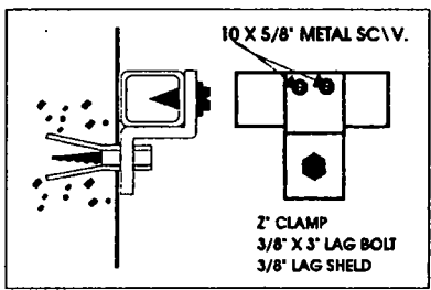
FRAME TO WALL ANCHOR DETAIL
