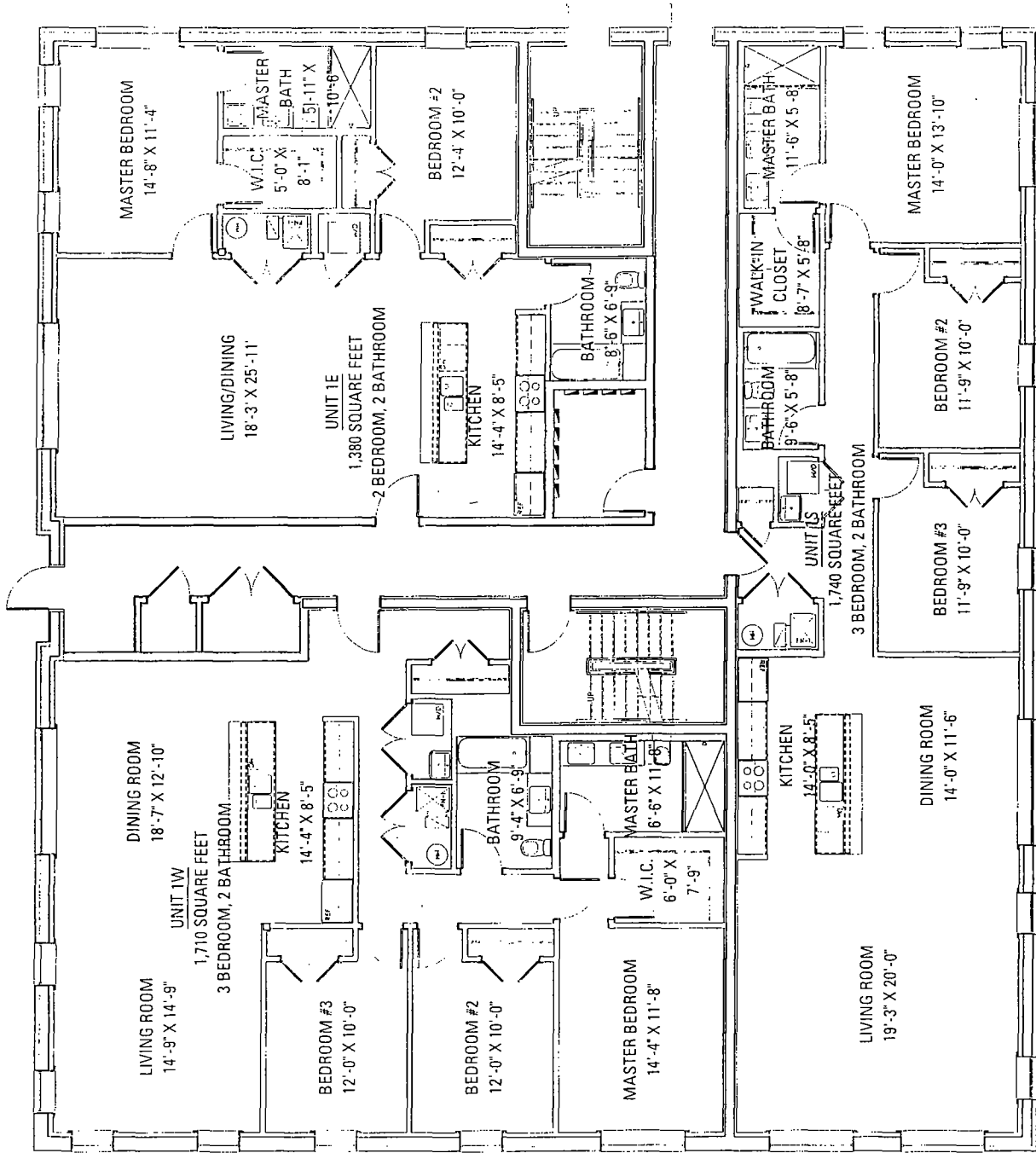
FIRST FLOOR 4155 W MELROSE PLANS 3/32" = 1'-0"
