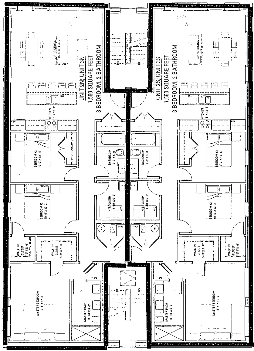
SECOND/THIRD FLOOR 3202 N KILDARE PLANS 3/32" = 1'-0"
