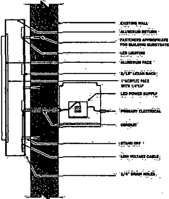
Reverse Channel - LED Halo Illuminated with 1" PUSHED-THRU ACRYLIC FACE
