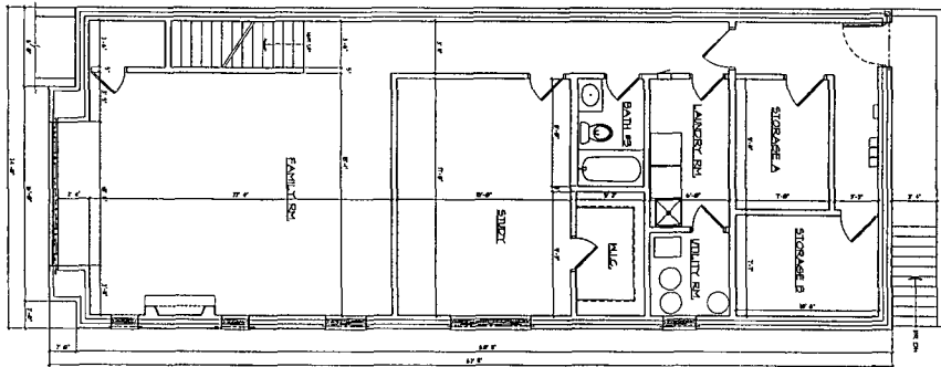
BASEMENT PLAN SCALE 1/8"=1'-0"
