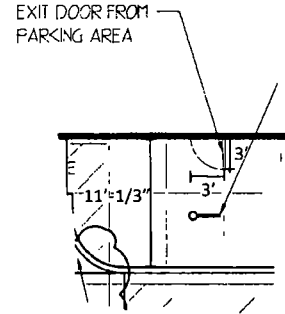
Typical Detail (emergency exits only)
