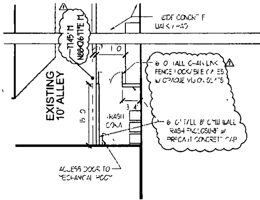
4 Trash enclosure 15' x 10'-3"
