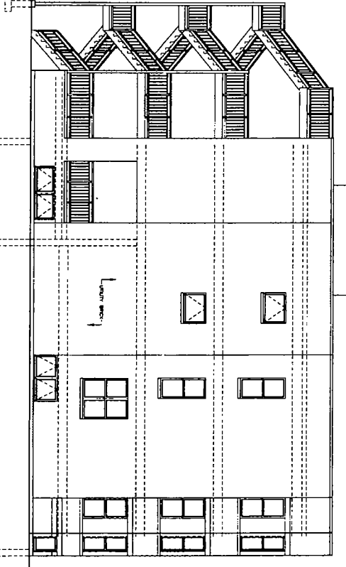
⊖ WEST ELEVATION SCALE 3/16" = 1'-0"
