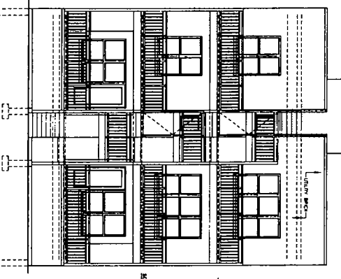
⊖ NORTH ELEVATION SCALE 3/16" = 1'-0"
