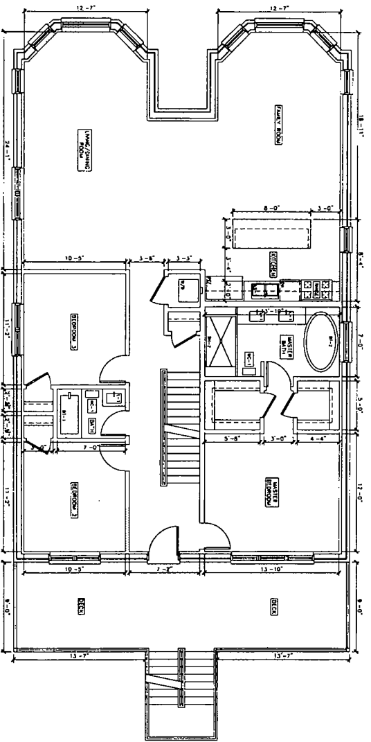
⊕ SECOND FLOOR PLAN SCALE 1/4" = 1'-0"
