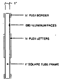
CROSS SECTION NTS
