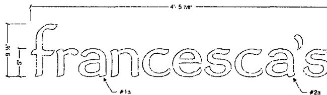
ECO LETTER DETAIL SCALE 1 1/2" = 1'-0"
