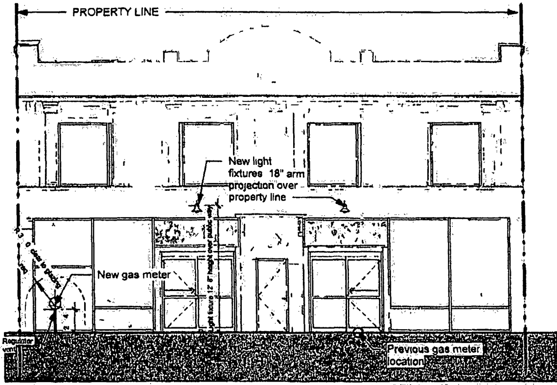
① PWU - North Elevation 1/8" = 1'-0"
