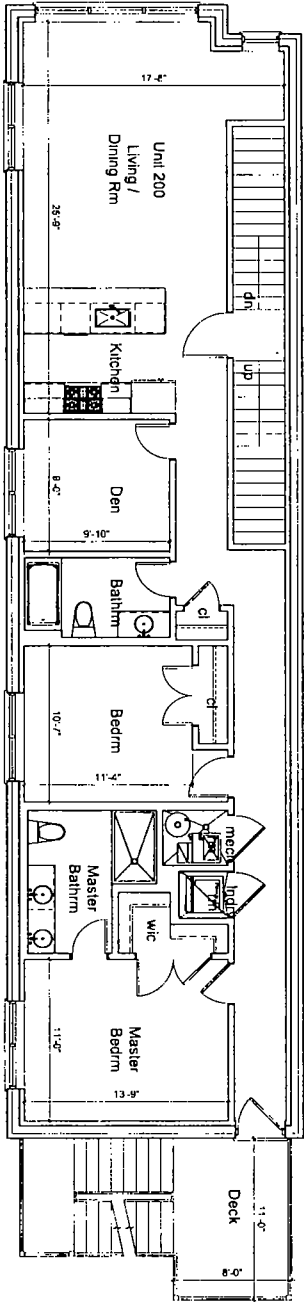
1 2nd Floor Plan
