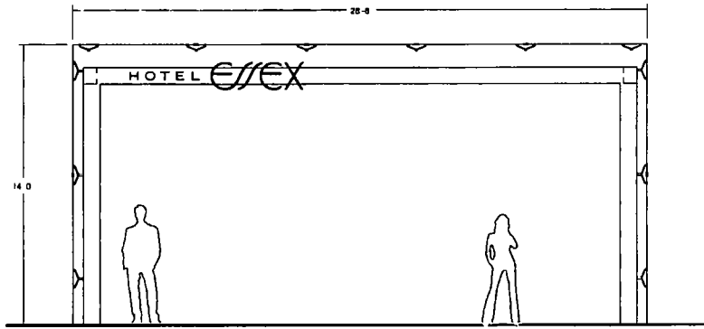
Elevation Scale 1/4" = 1'
