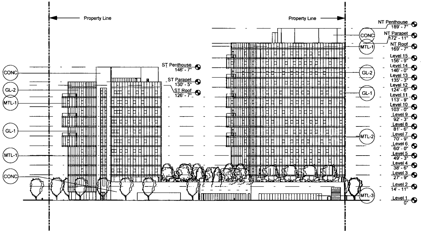
1 PD - East Elevation 1" = 60'-0"
