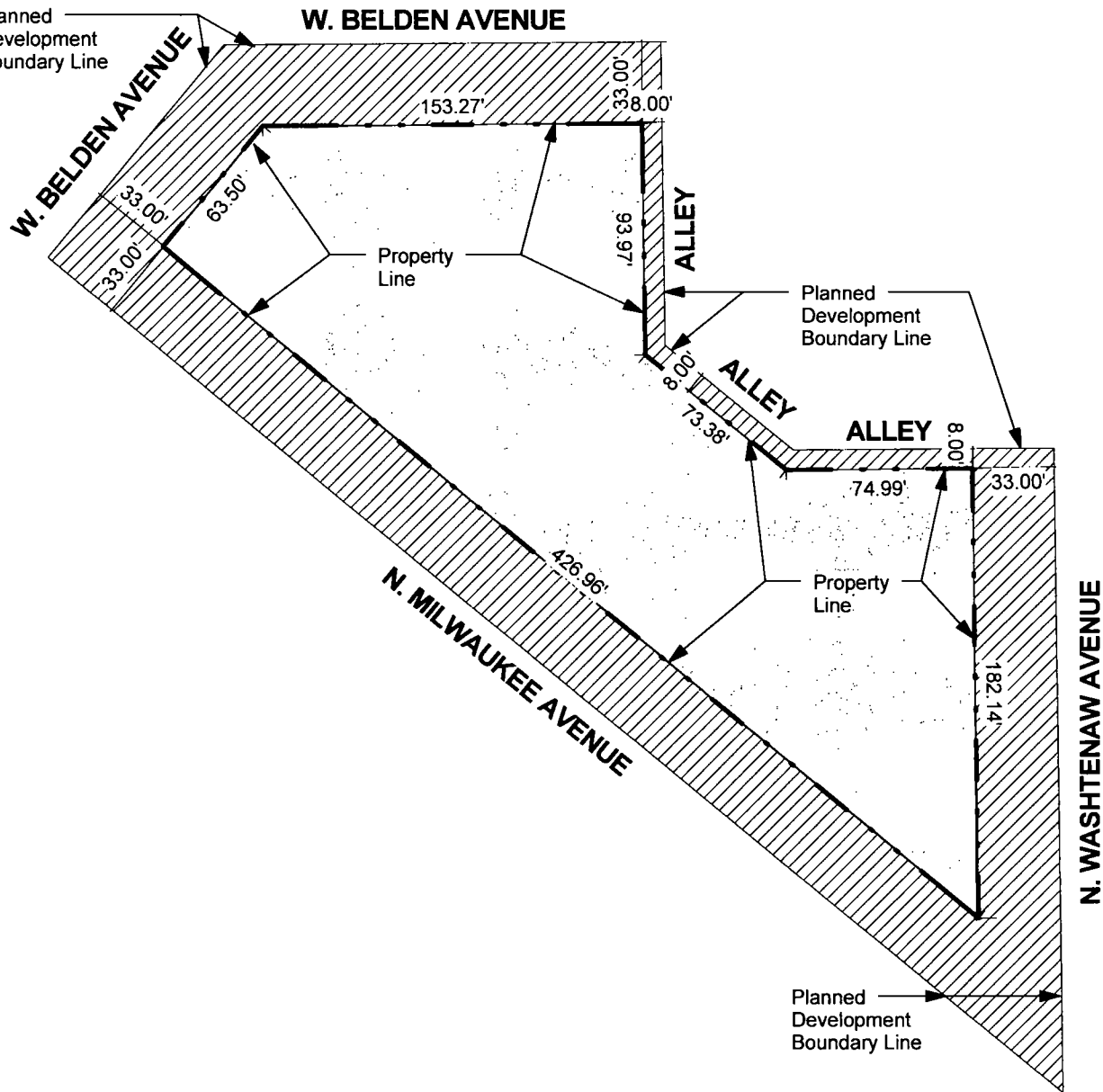
① PD - Boundary and Property Line Map 1/64" = 1'-0"
