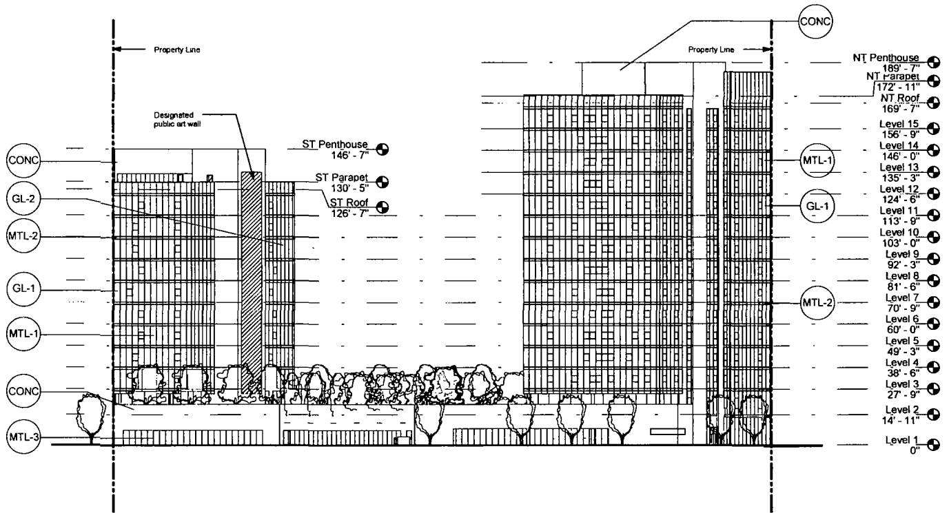
① PD - North Elevation 1" = 60'-0"
