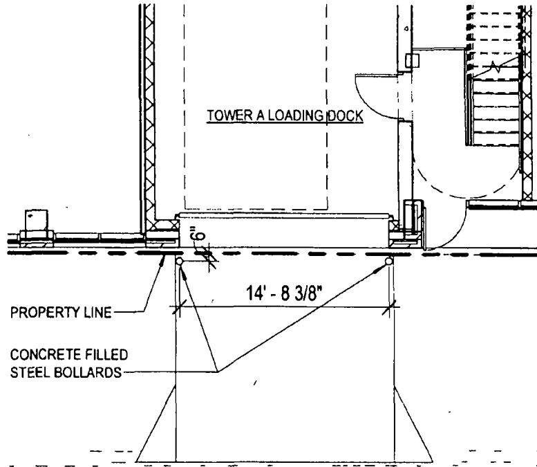
TOWER A PLAN
