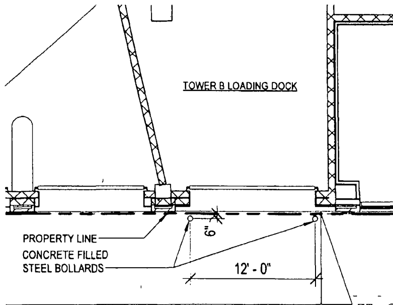
TOWER B PLAN
