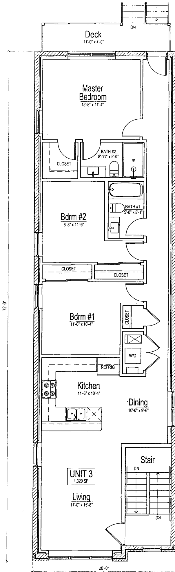
3RD FLOOR PLAN 3920-32 S. Calumet Ave Chicago, Illinois
