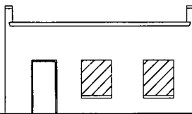
② PROPOSED SOUTH ELEVATION SCALE 3/16" = 1'-0"
