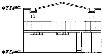
① PROPOSED NORTH ELEVATION SCALE 3/16" = 1'-0"
